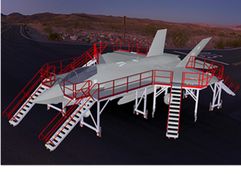
F-35 Docking Stand A fully surrounding platform that allows access to all areas simultaneously, with unique advantages like self-levelling stairs and height adjustment in the dock to suit different ramp loadings of the F35.
